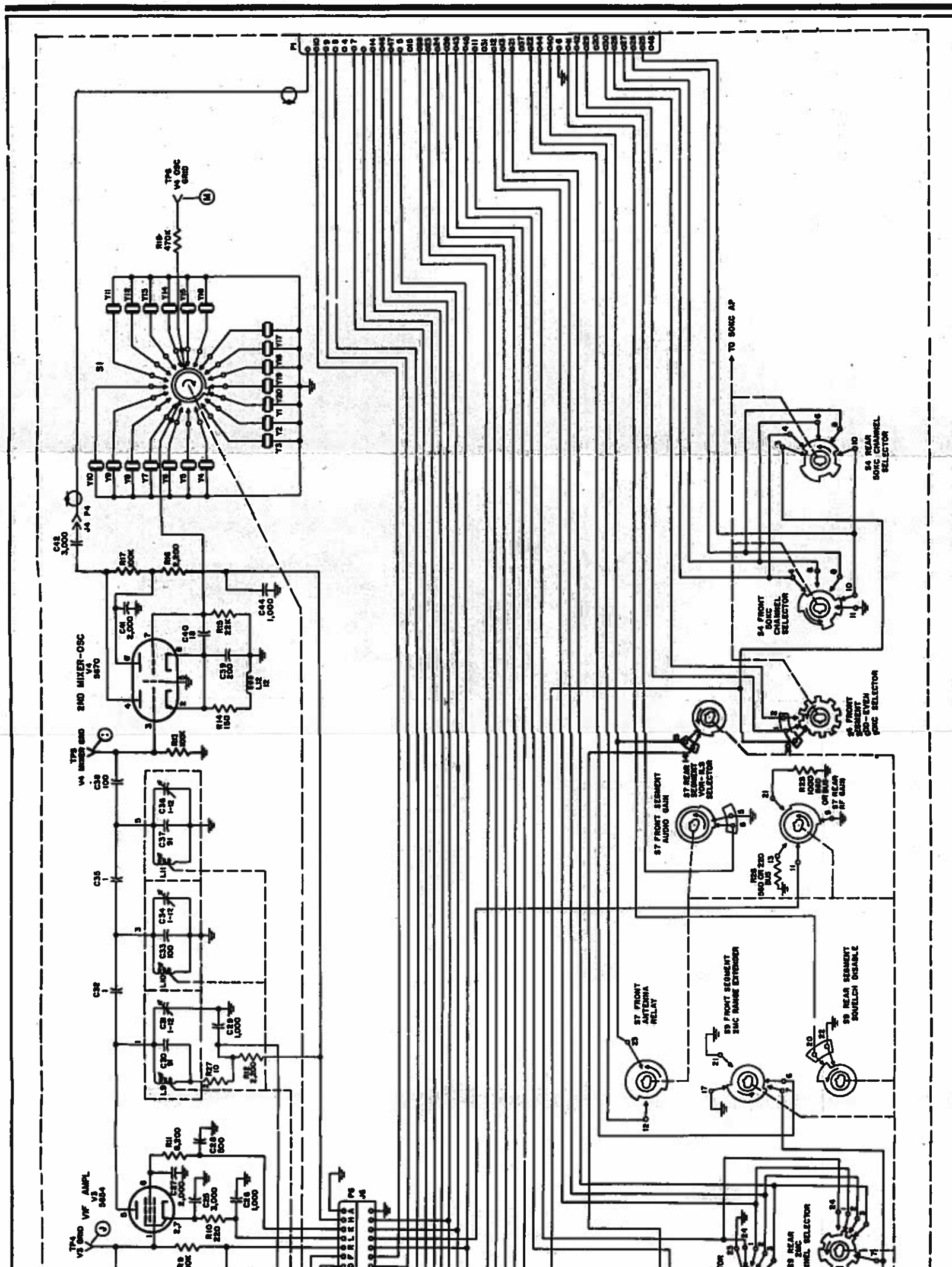
Figure 7-43. VHF Navigation and Communications Receiver 51X-2B (Units through MCN 7867) Schematic Diagram (Sheet 1 of 3)
